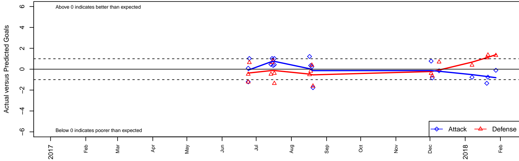
Snohomish United Black G03 Dots are actual minus expected GF (blue circles) and GA (red triangles). Blue line is smoothed change in attack strength. Red is smoothed change in defense strength.
